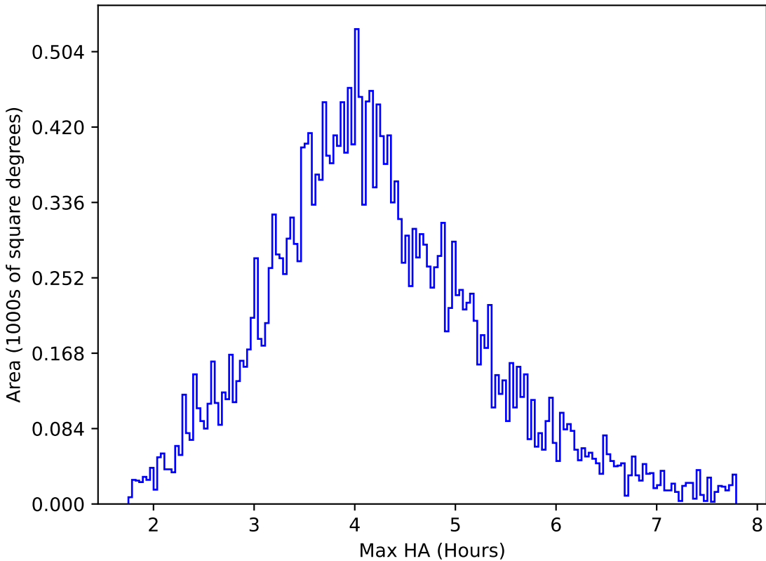
too_5_1v3.4_10yrs All sky r band: Max HA
