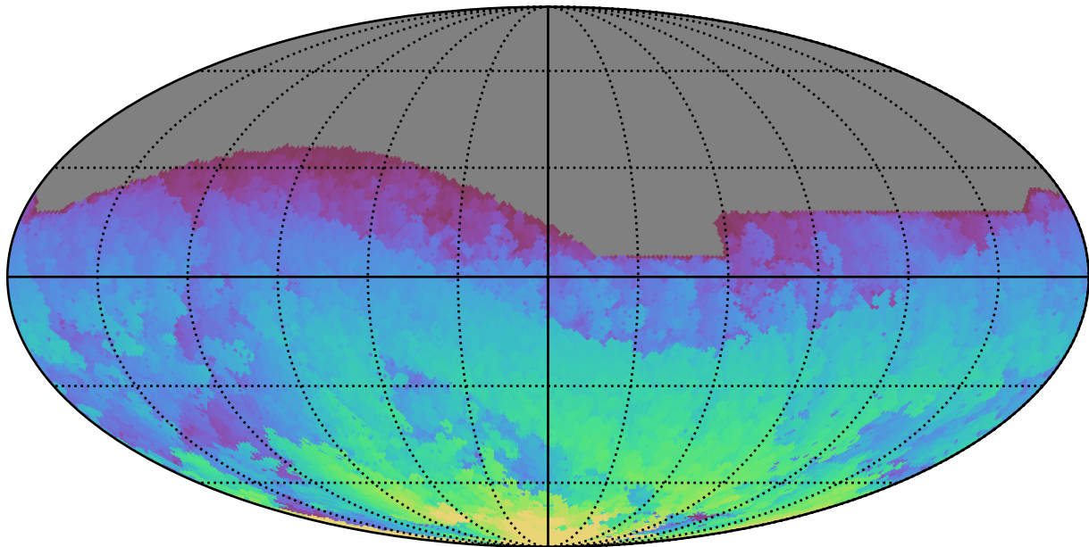
too_5_1v3.4_10yrs All sky i band: Max HA
