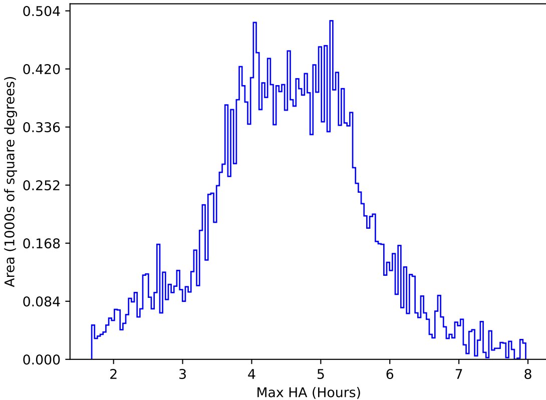
too_5_1v3.4_10yrs All sky i band: Max HA
