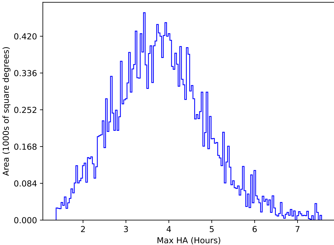
too_5_1v3.4_10yrs All sky g band: Max HA
