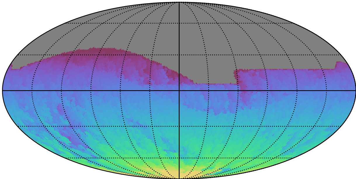
too_5_1v3.4_10yrs All sky all bands: Max HA
