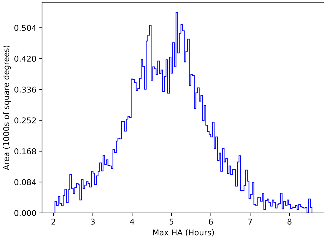
too_5_1v3.4_10yrs All sky all bands: Max HA
