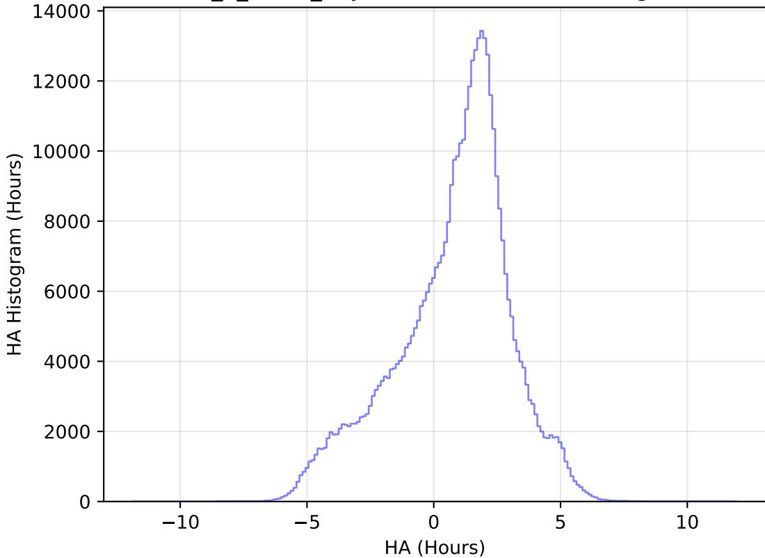
too_5_1v3.4_10yrs WFD z band: HA Histogram
