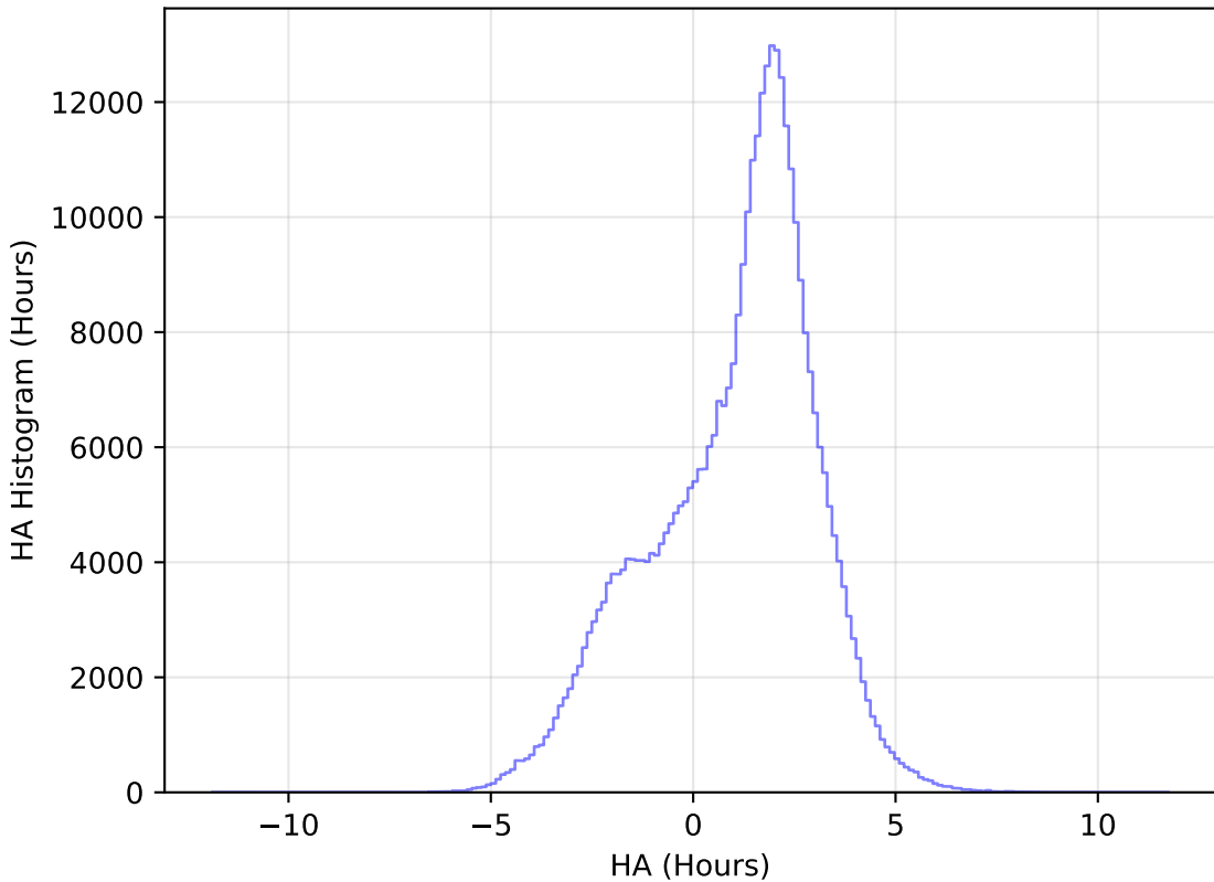
too_5_1v3.4_10yrs WFD y band: HA Histogram
