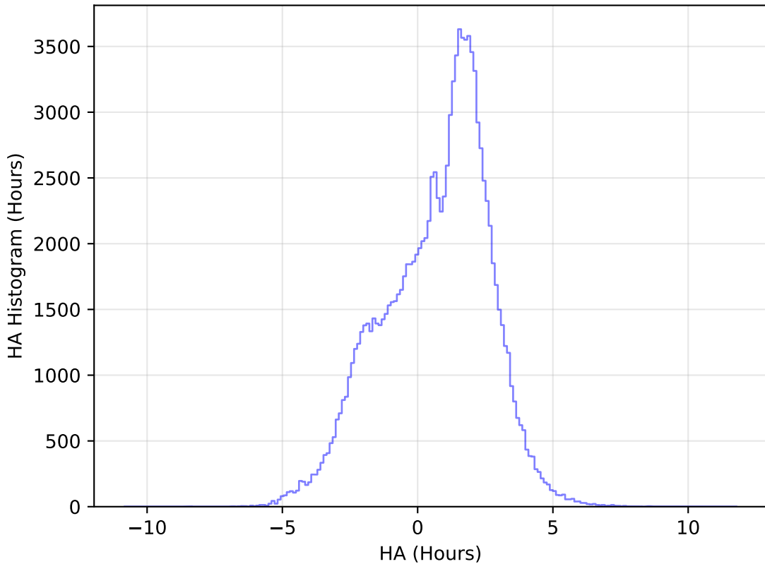
too_5_1v3.4_10yrs WFD u band: HA Histogram
