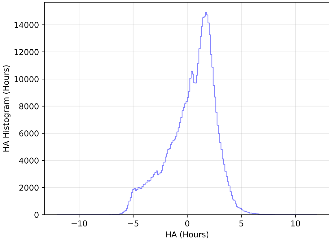
too_5_1v3.4_10yrs WFD r band: HA Histogram
