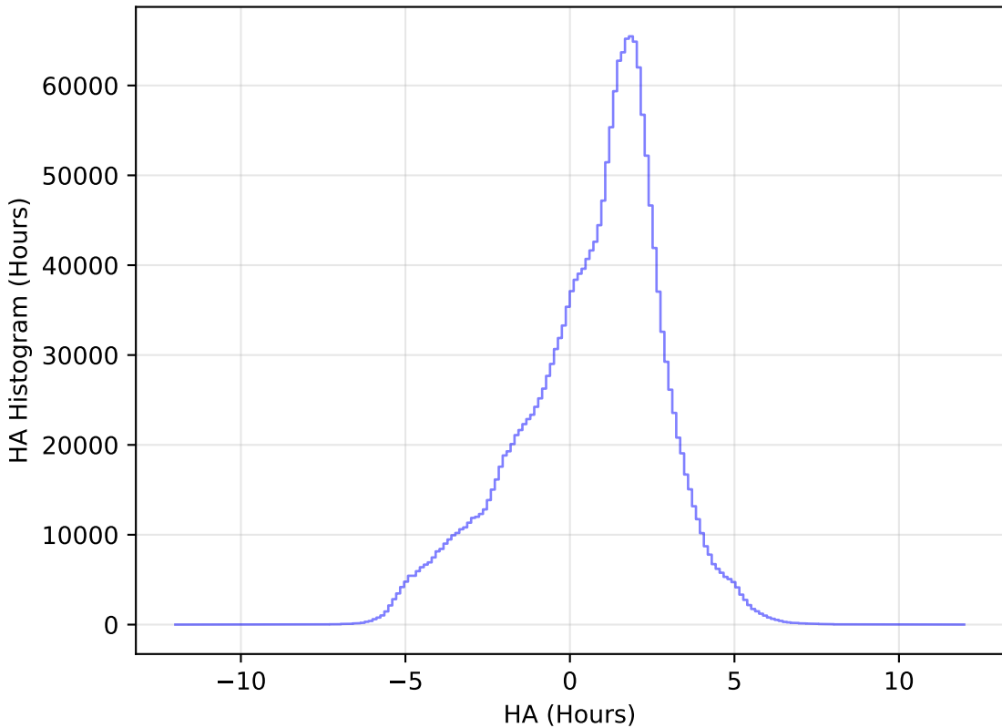
too_5_1v3.4_10yrs WFD all bands: HA Histogram
