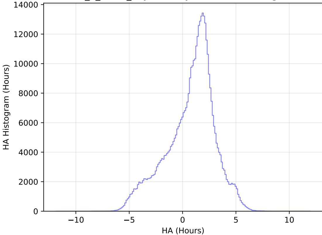
too_5_1v3.4_10yrs All sky z band: HA Histogram
