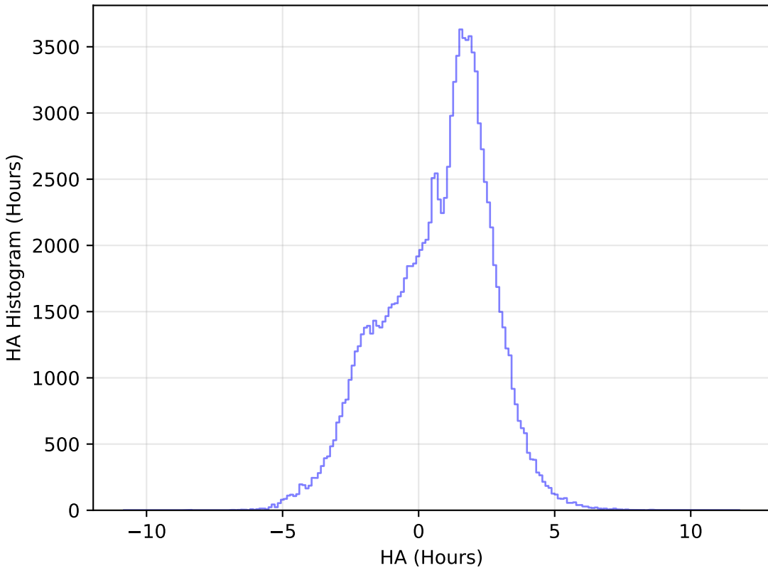
too_5_1v3.4_10yrs All sky u band: HA Histogram
