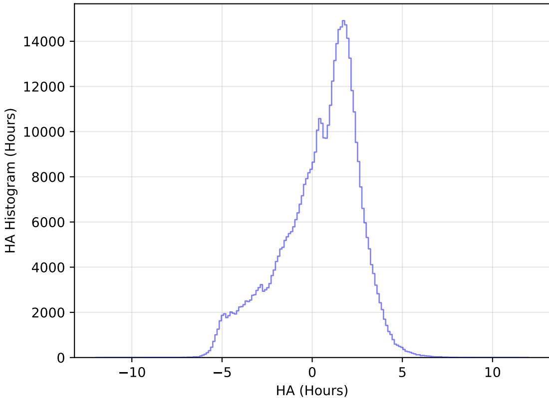
too_5_1v3.4_10yrs All sky r band: HA Histogram
