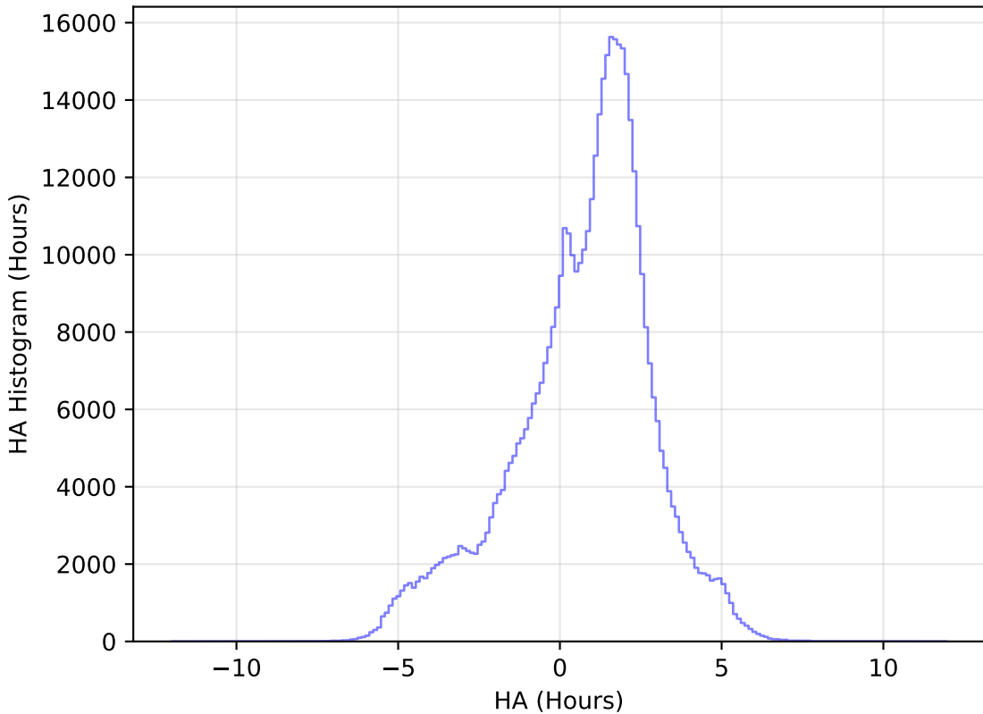
too_5_1v3.4_10yrs All sky i band: HA Histogram
