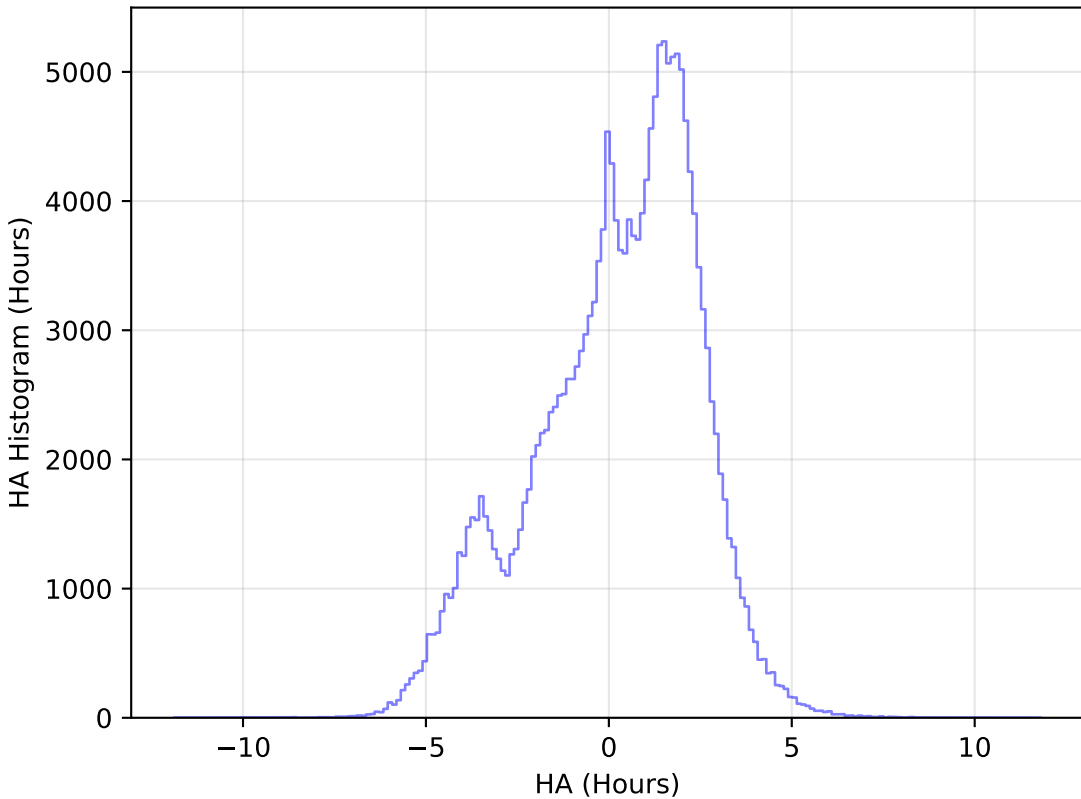
too_5_1v3.4_10yrs All sky g band: HA Histogram
