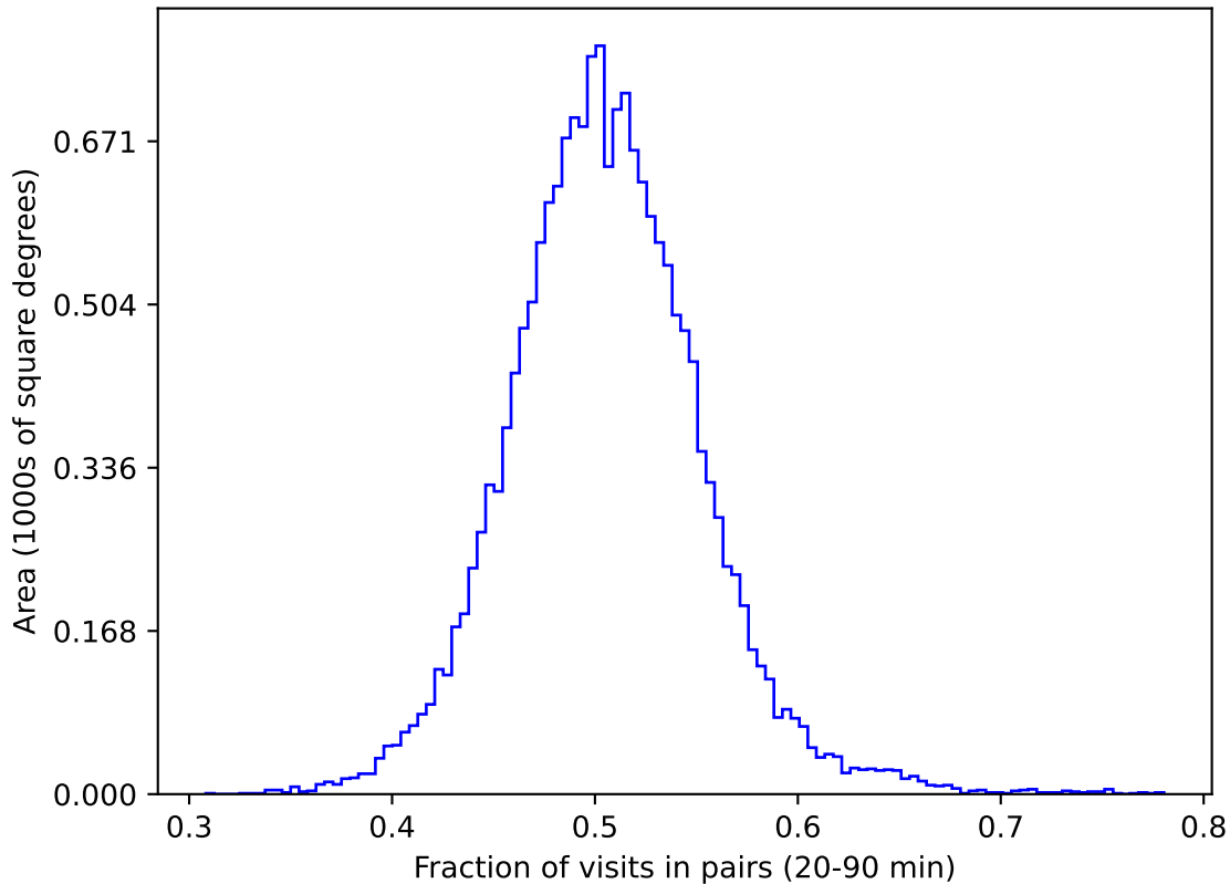
too_5_1v3.4_10yrs gri WFD: Fraction of visits in pairs (20-90 min)
