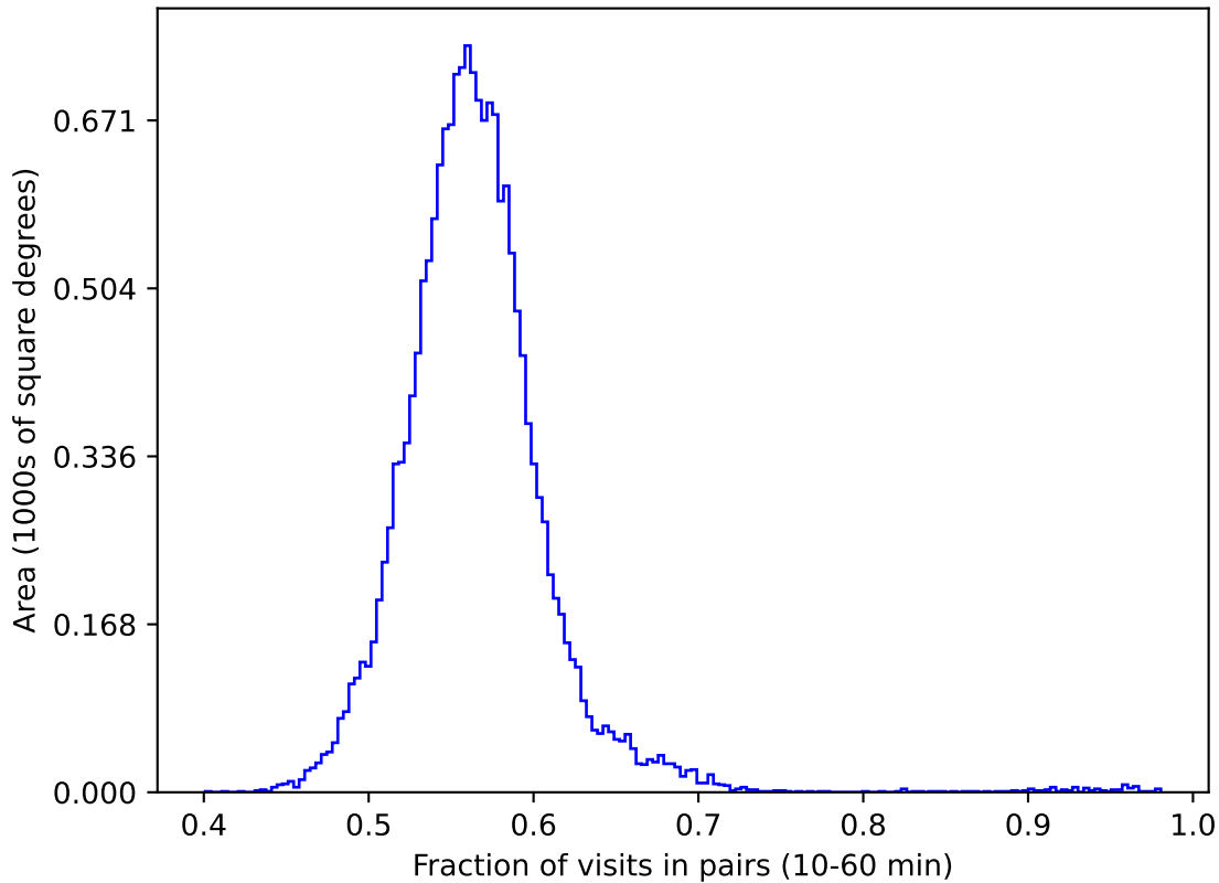
too_5_1v3.4_10yrs gri WFD: Fraction of visits in pairs (10-60 min)
