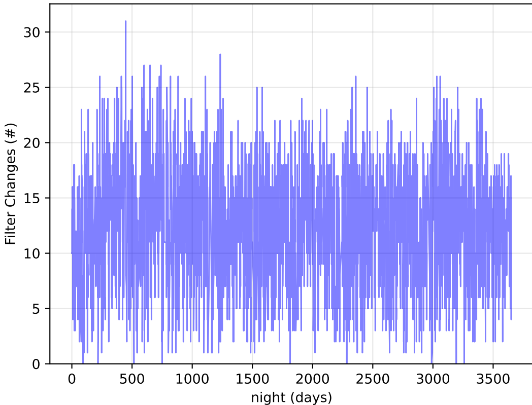
too_5_1v3.4_10yrs Per Night: Filter Changes
