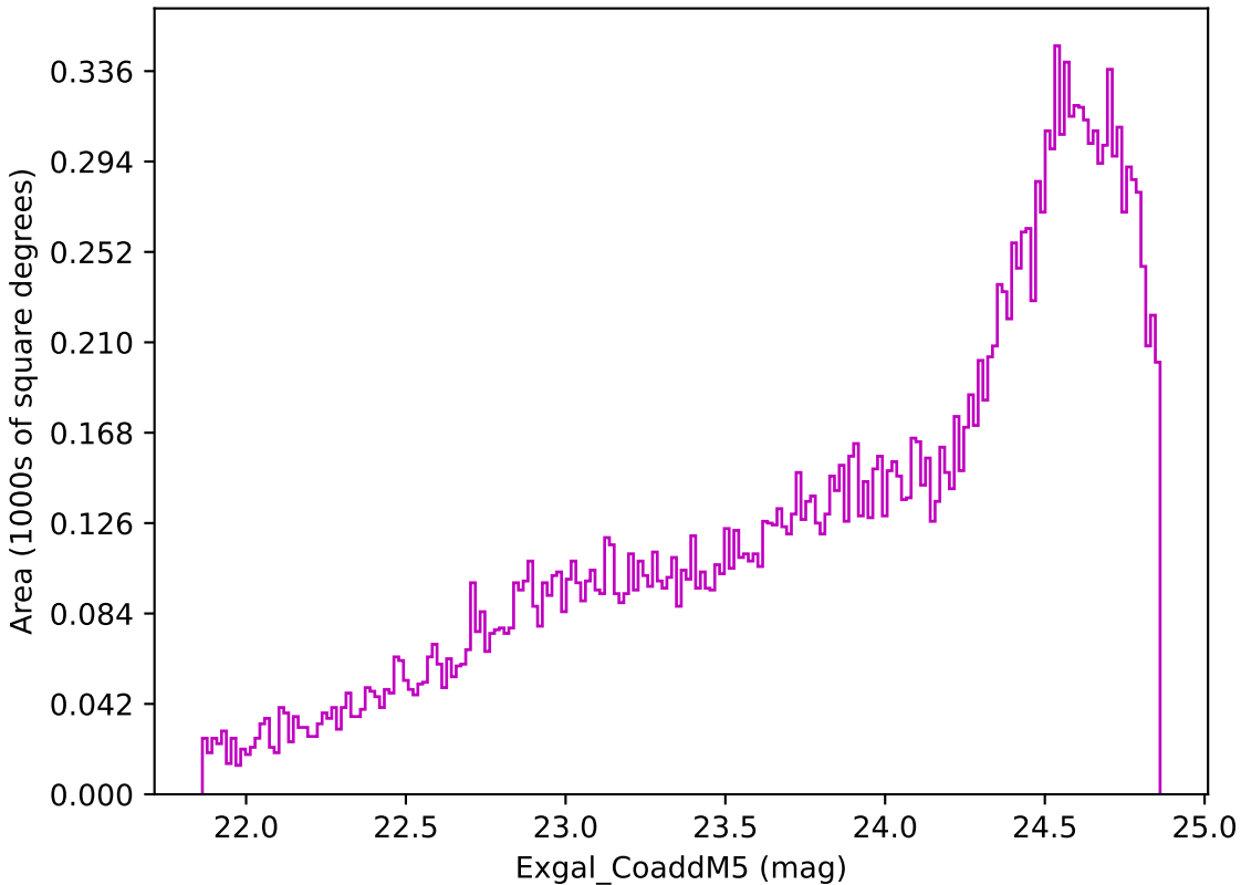
too_5_1v3.4_10yrs Yr 3-4 z band: Exgal_CoaddM5
