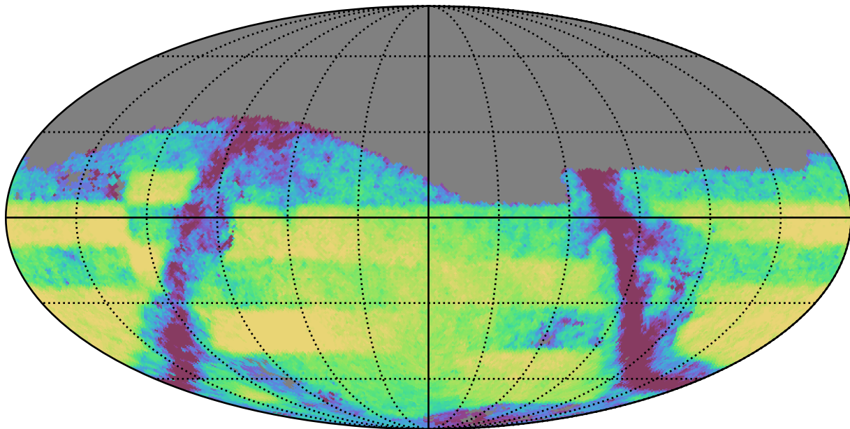
too_5_1v3.4_10yrs Yr 3-4 i band: Exgal_CoaddM5
