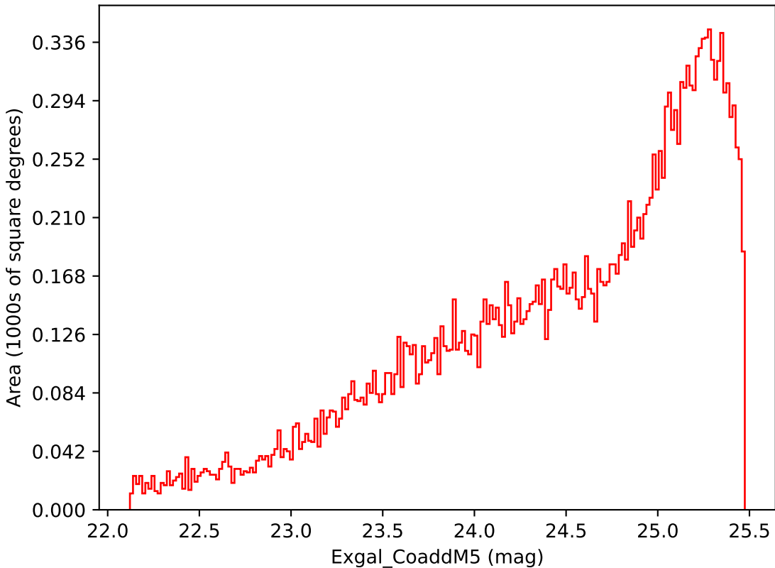
too_5_1v3.4_10yrs Yr 3-4 i band: Exgal_CoaddM5
