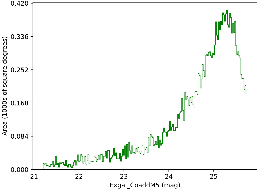
too_5_1v3.4_10yrs Yr 3-4 g band: Exgal_CoaddM5
