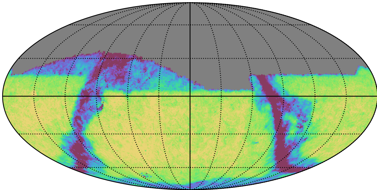
too_5_1v3.4_10yrs Yr 1 z band: Exgal_CoaddM5
