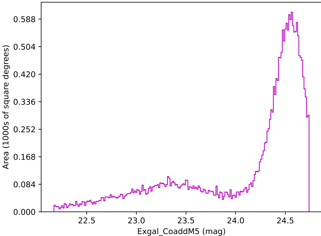
too_5_1v3.4_10yrs Yr 1 z band: Exgal_CoaddM5
