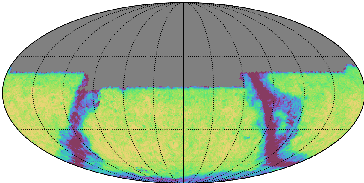
too_5_1v3.4_10yrs Yr 1 y band: Exgal_CoaddM5
