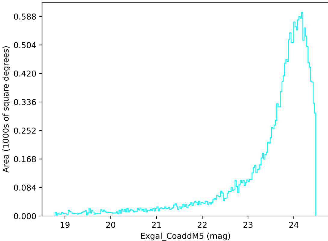
too_5_1v3.4_10yrs Yr 1 u band: Exgal_CoaddM5
