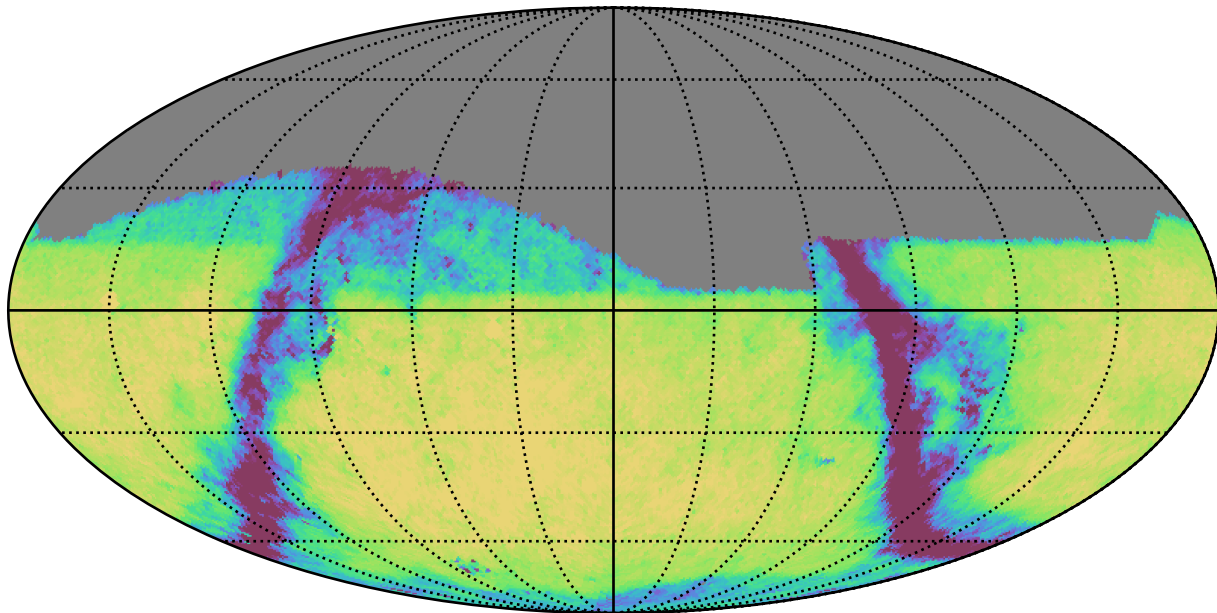
too_5_1v3.4_10yrs Yr 1 r band: Exgal_CoaddM5
