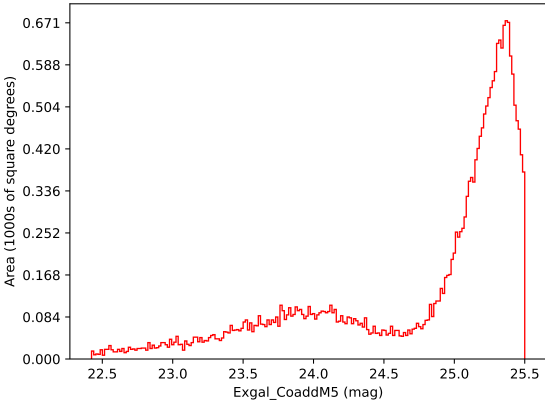
too_5_1v3.4_10yrs Yr 1 i band: Exgal_CoaddM5
