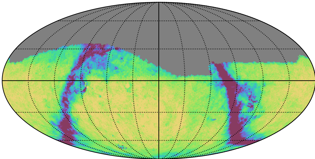
too_5_1v3.4_10yrs Yr 1 g band: Exgal_CoaddM5
