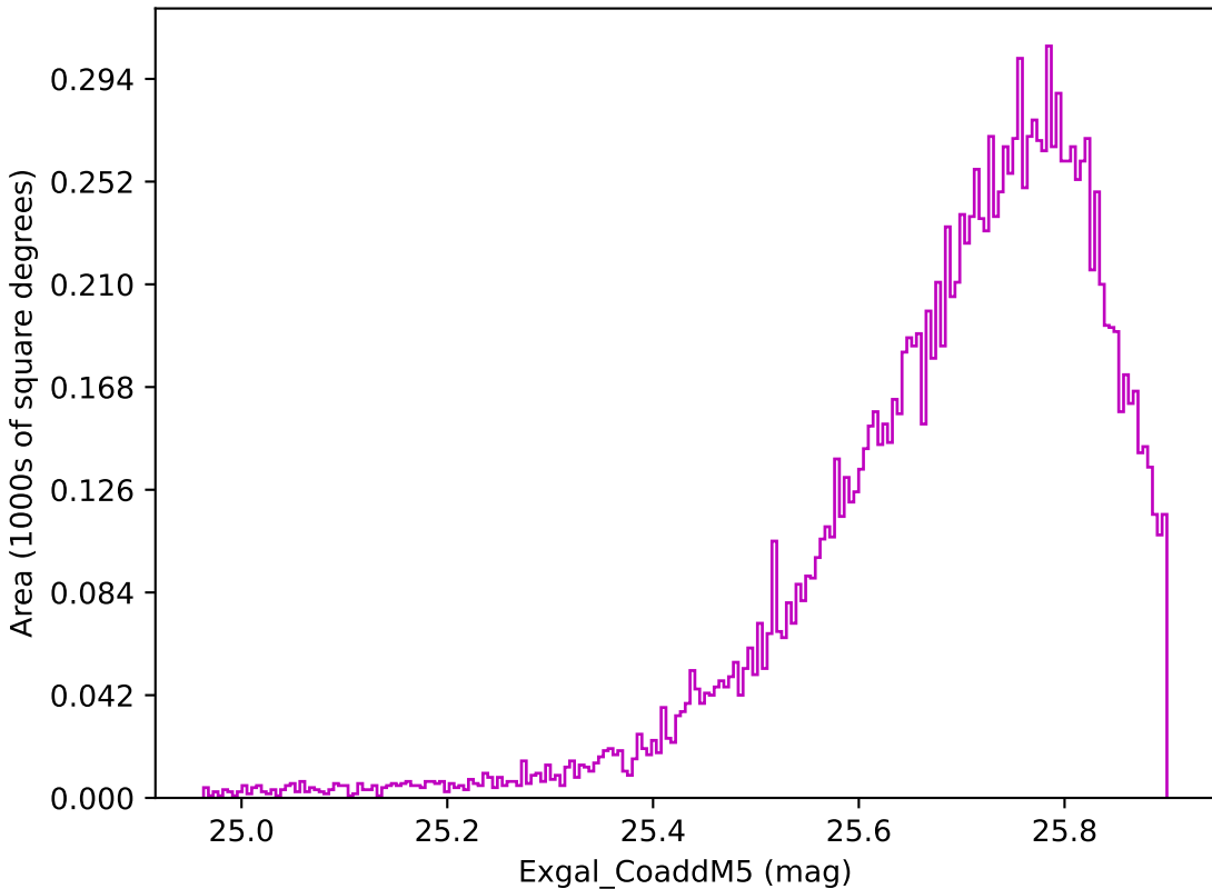
too_5_1v3.4_10yrs WFD z band: Exgal_CoaddM5
