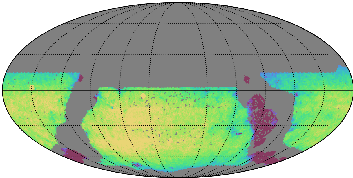
too_5_1v3.4_10yrs WFD y band: Exgal_CoaddM5
