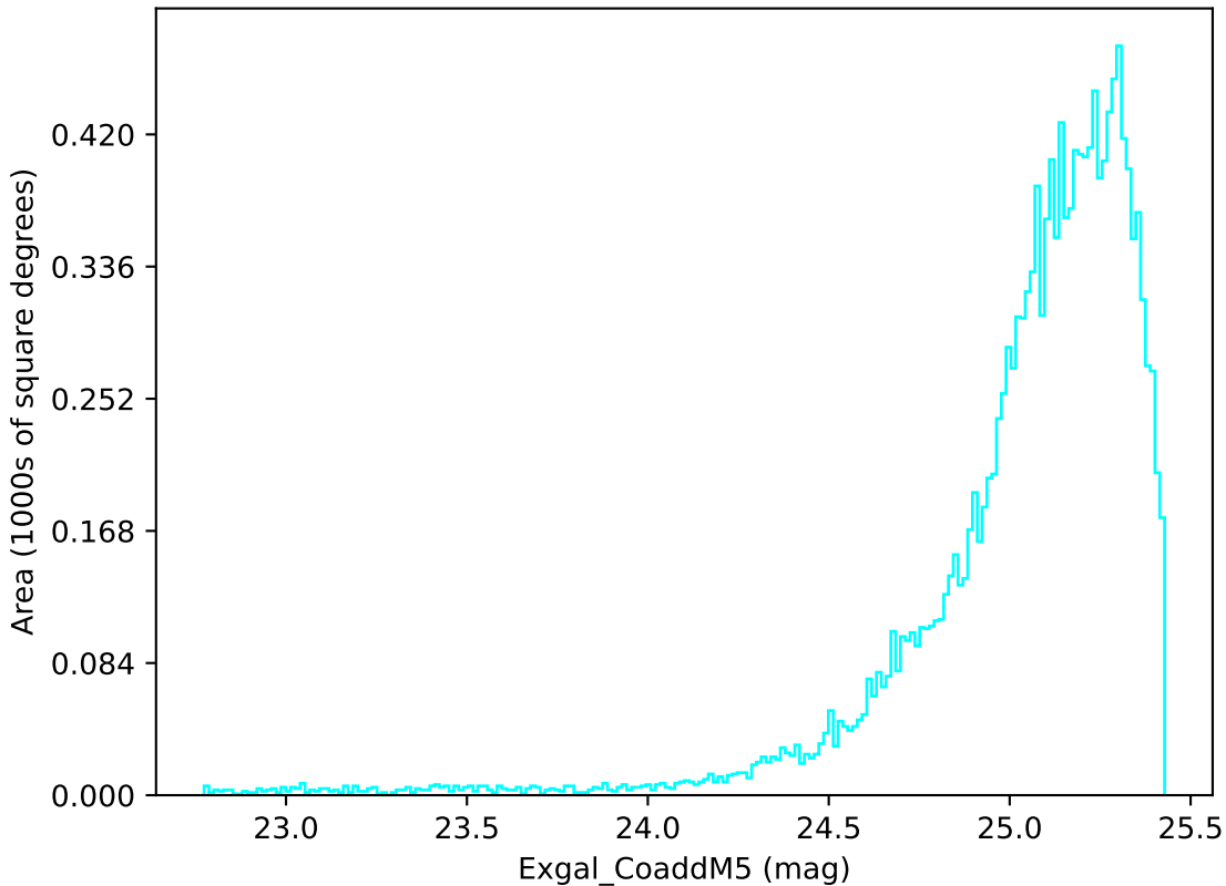
too_5_1v3.4_10yrs WFD u band: Exgal_CoaddM5
