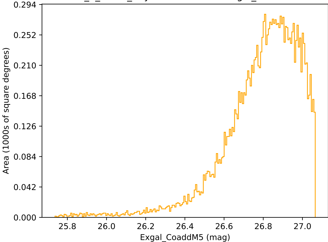
too_5_1v3.4_10yrs WFD r band: Exgal_CoaddM5
