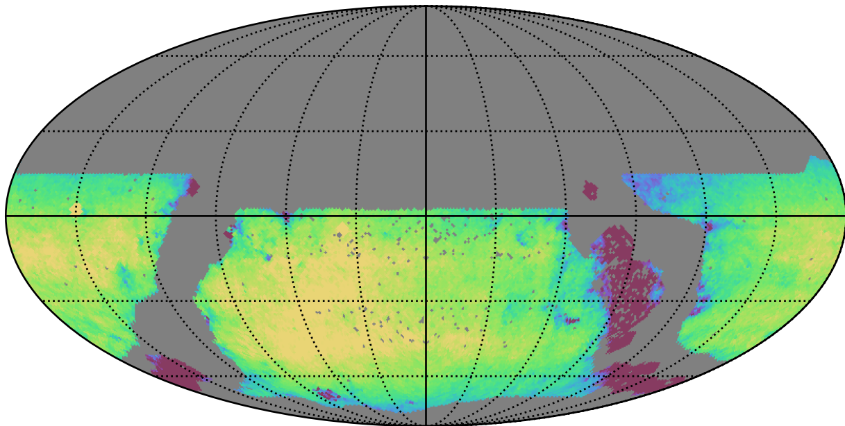
too_5_1v3.4_10yrs WFD i band: Exgal_CoaddM5
