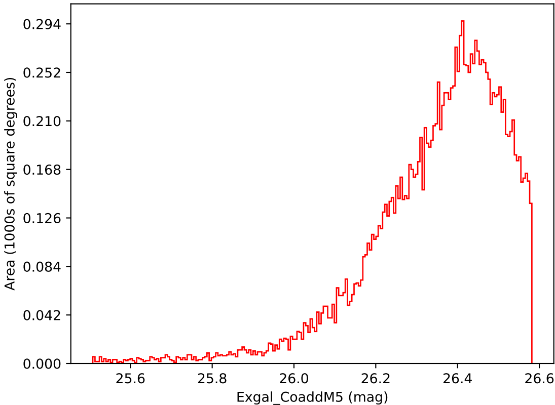
too_5_1v3.4_10yrs WFD i band: Exgal_CoaddM5
