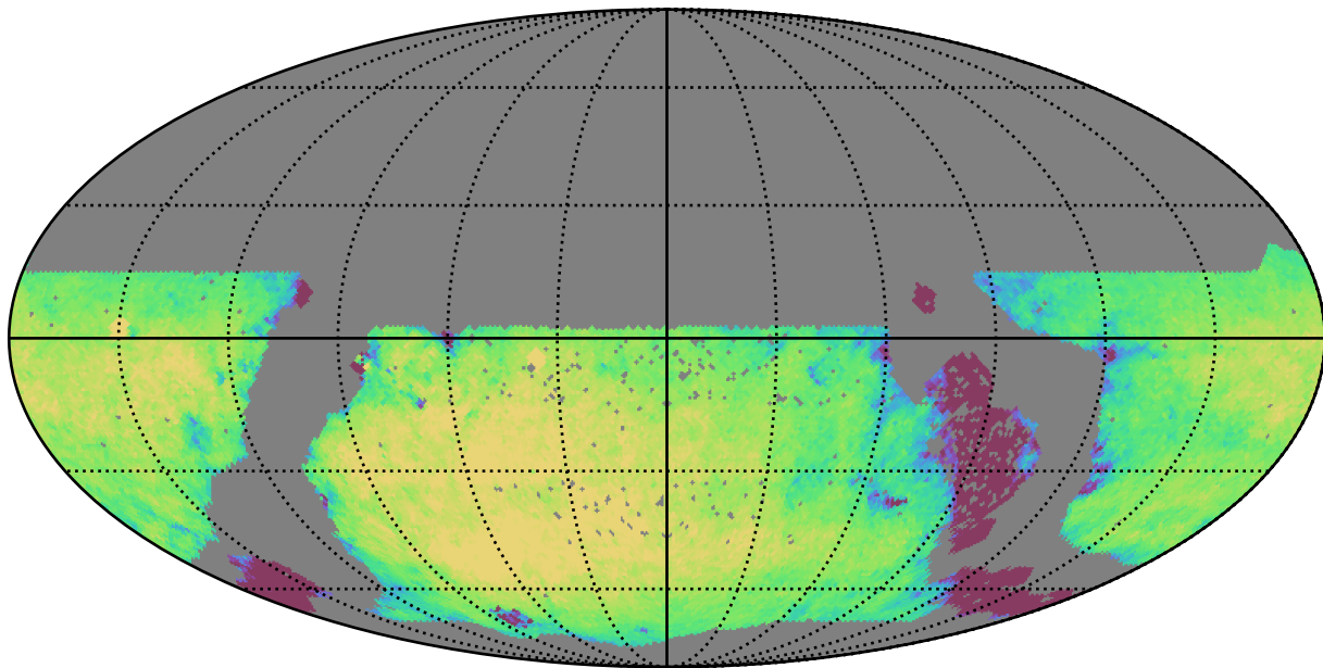
too_5_1v3.4_10yrs WFD g band: Exgal_CoaddM5
