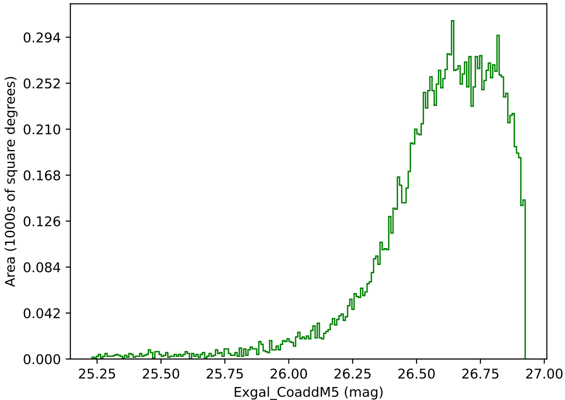
too_5_1v3.4_10yrs WFD g band: Exgal_CoaddM5
