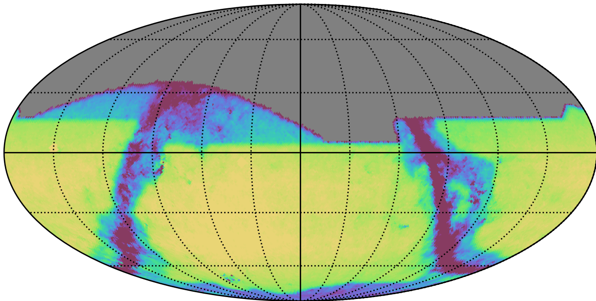
too_5_1v3.4_10yrs All sky z band: Exgal_CoaddM5
