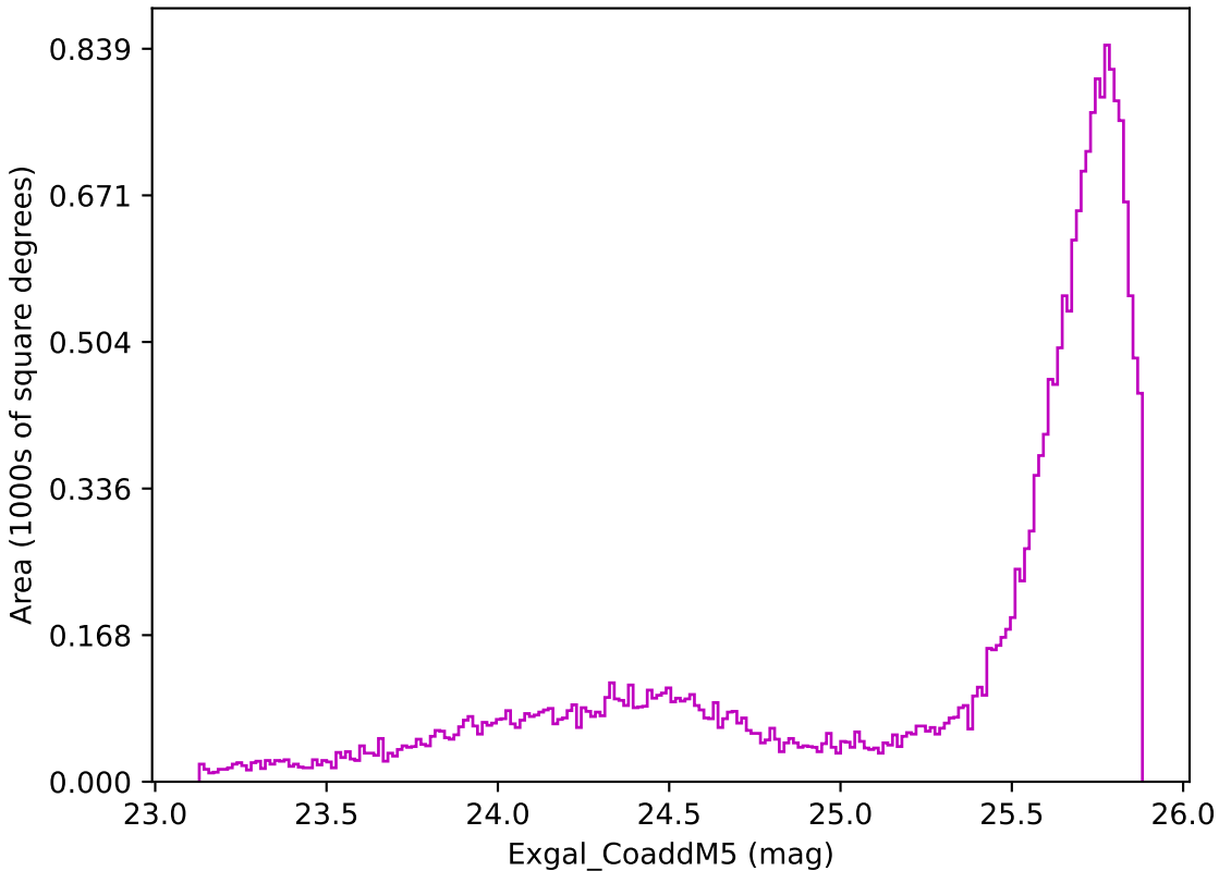
too_5_1v3.4_10yrs All sky z band: Exgal_CoaddM5
