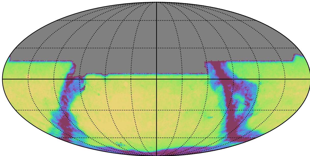
too_5_1v3.4_10yrs All sky y band: Exgal_CoaddM5
