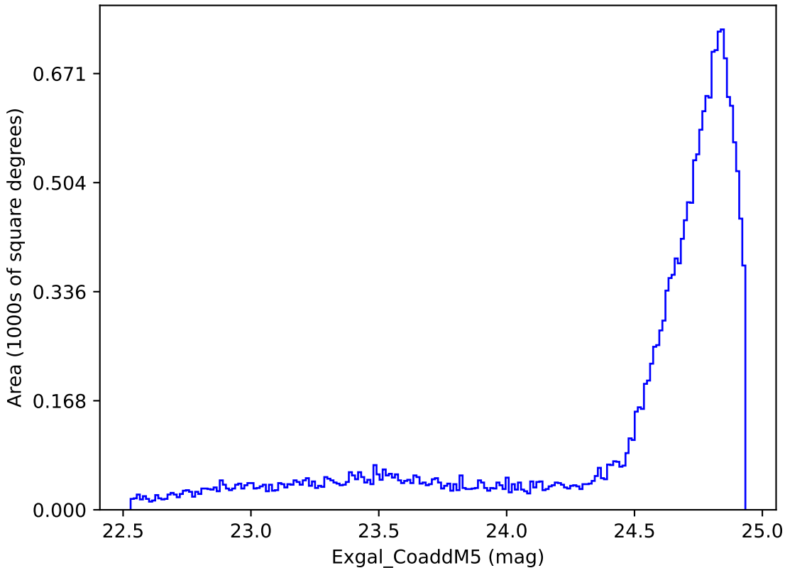
too_5_1v3.4_10yrs All sky y band: Exgal_CoaddM5
