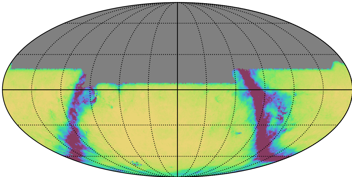
too_5_1v3.4_10yrs All sky u band: Exgal_CoaddM5
