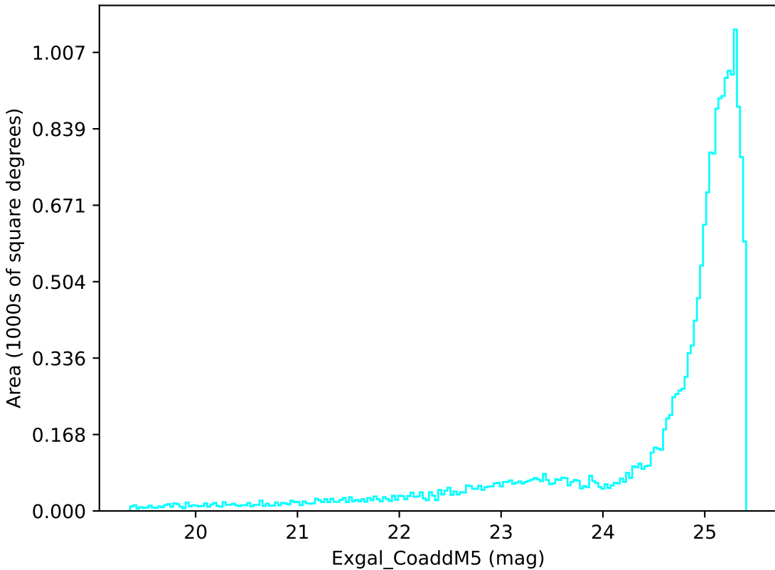
too_5_1v3.4_10yrs All sky u band: Exgal_CoaddM5
