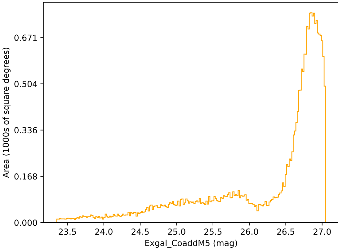
too_5_1v3.4_10yrs All sky r band: Exgal_CoaddM5
