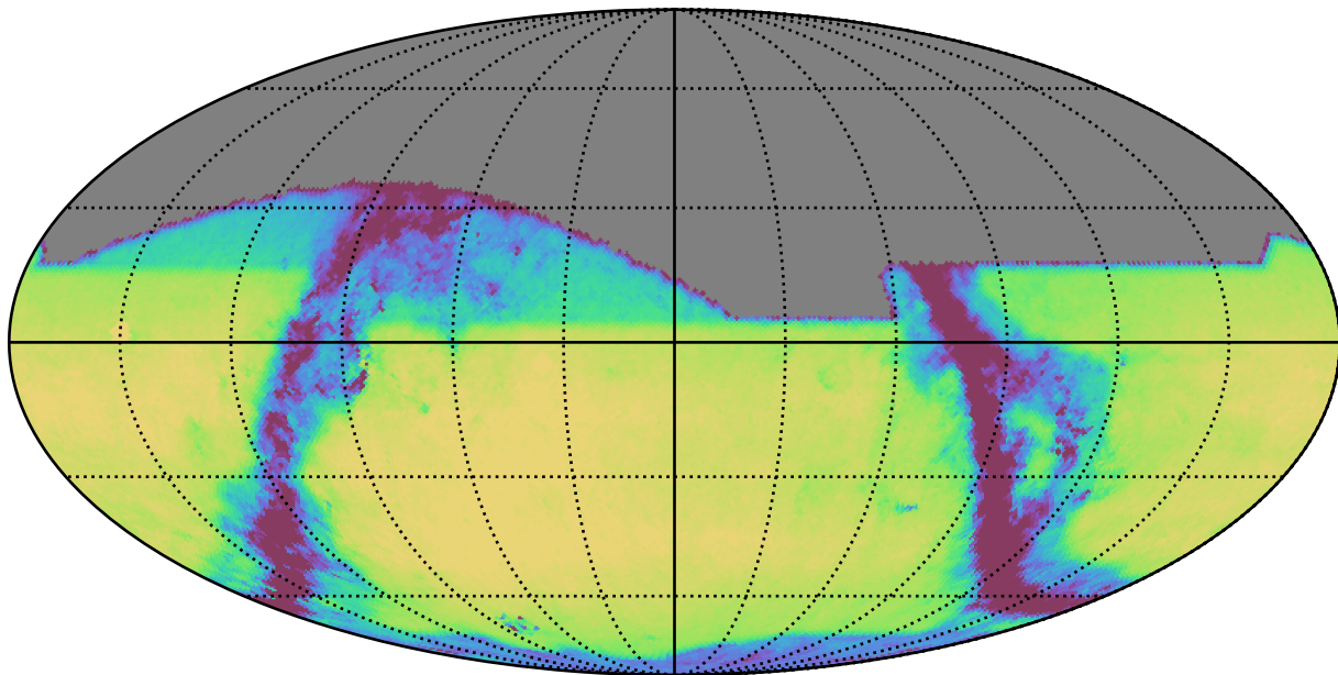
too_5_1v3.4_10yrs All sky i band: Exgal_CoaddM5
