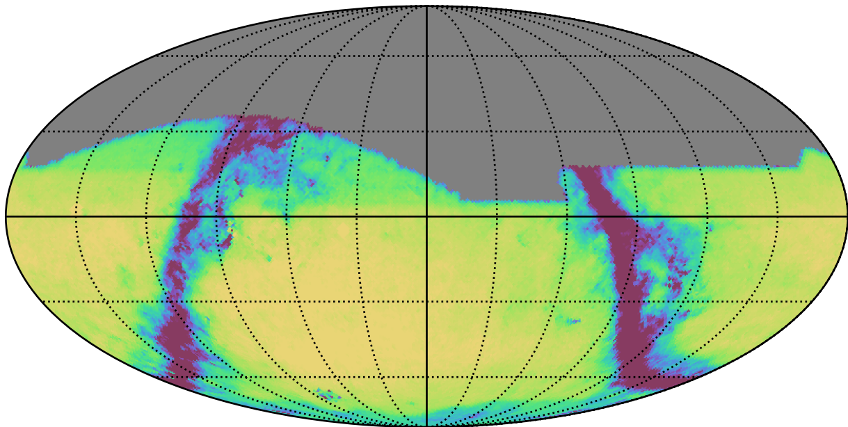
too_5_1v3.4_10yrs All sky g band: Exgal_CoaddM5
