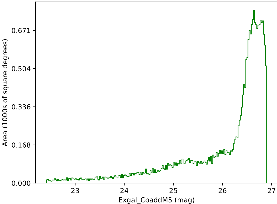
too_5_1v3.4_10yrs All sky g band: Exgal_CoaddM5
