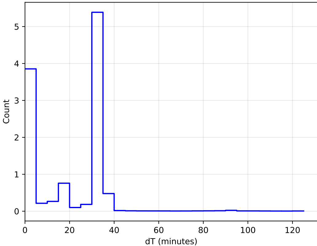
1e6 too_5_1v3.4_10yrs WFD: DeltaT Histogram
