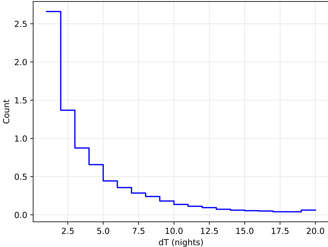
too_5_1v3.4_10yrs WFD all bands: DeltaNight Histogram 1e6
